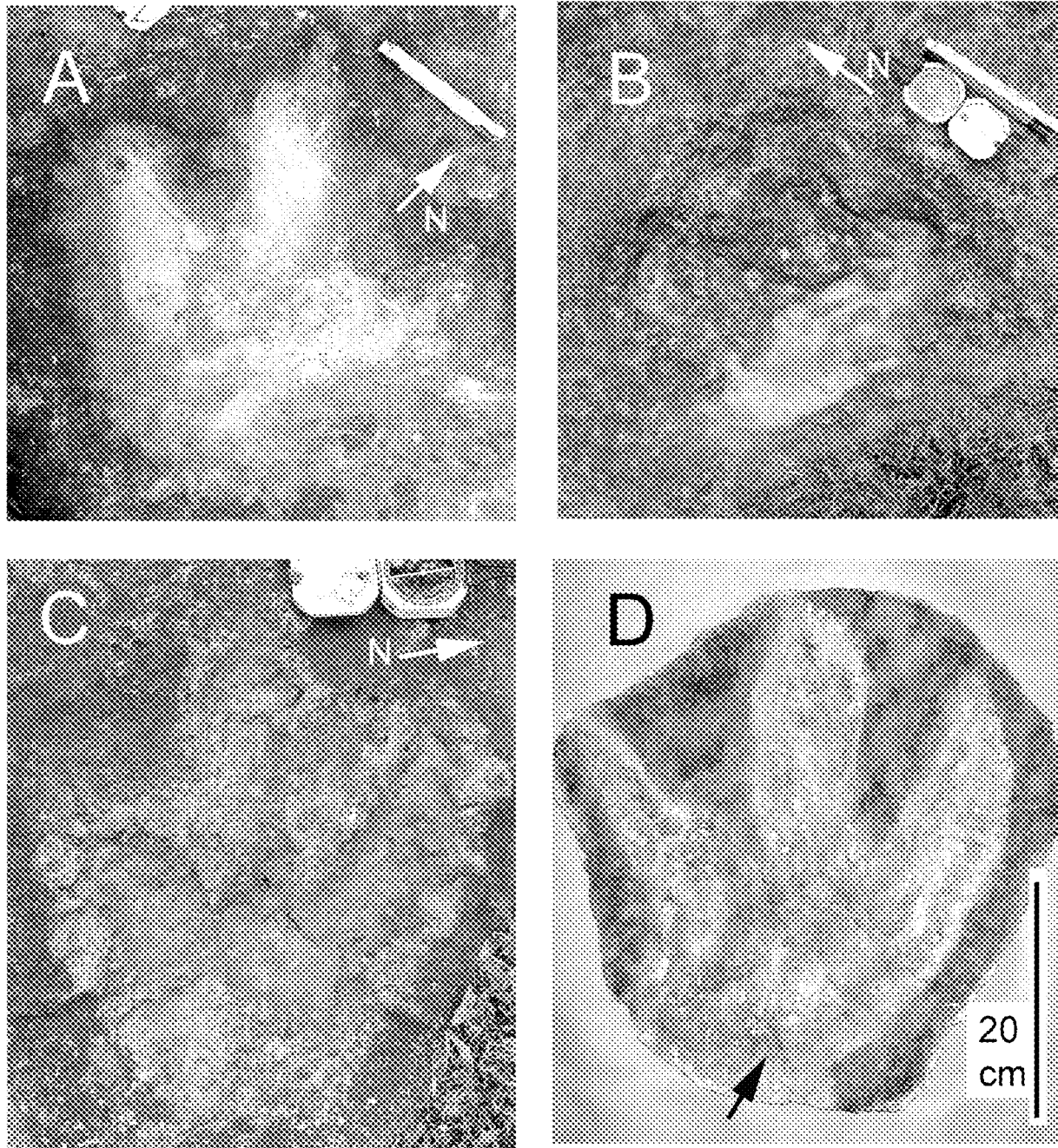
FIG. 4. A, Track number 7 (see Fig. 6), one of most well-preserved tracks at site, showing well-developed tridactyl footprint. Scale in A and B is 20 cm long. B, Moderately-preserved track number 1 (see Fig. 6), which may be undertrack or transmitted print ( sensu Thulborn, 1990). C, Track number 17 (see Fig. 6), the best-preserved track at site. D, Painted plaster cast of track number 17, produced from silicone rubber mold. Track shows three, relatively broad digits and slightly bilobed posterior margin (black arrow). Scale is same in C and D.
